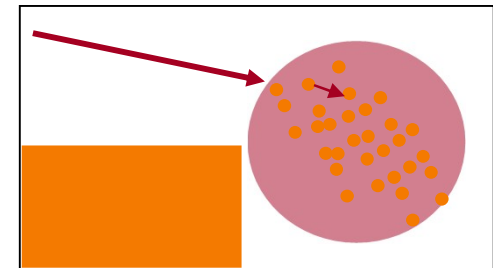
Scattering
