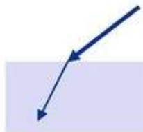
refraction
